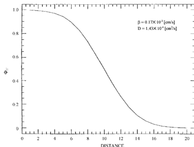
Fig. 7. Displacing fluid saturation as a function of position.
